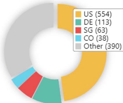
Top Countries
